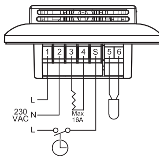
Anschlüsse OTN2-1991
