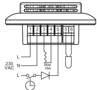
Anschlüsse OTD2-1999 (Frostschutzmodus)
