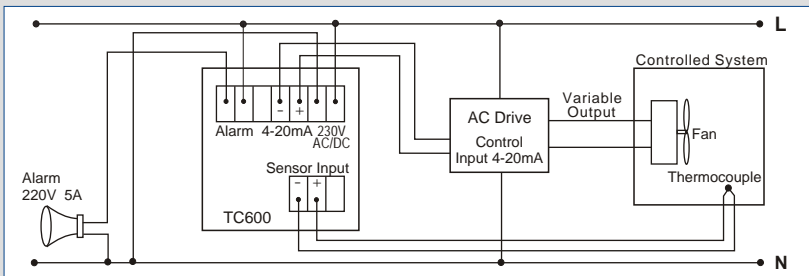
Example 3: Analogue control output (4-20mA) to a variable speed AC drive. Relay output for alarm. Input is from a thermocouple.
