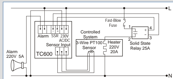
Example 2: Controller with Solid State Relay (SSR). Output and relay output for alarm. Input is from PT-100 RTD.
